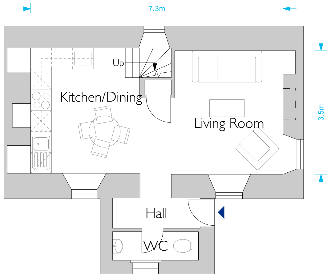
GROUND FLOOR
